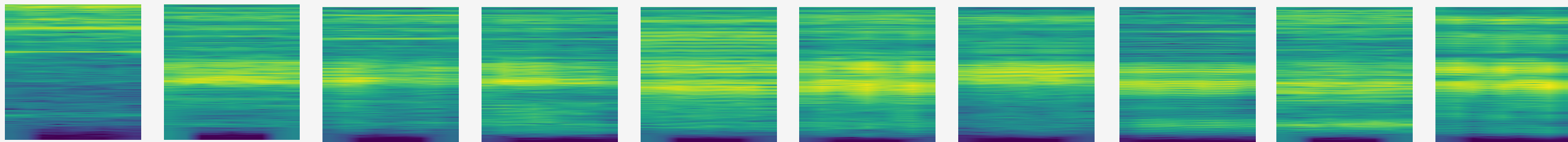
STFT Spectrograms
